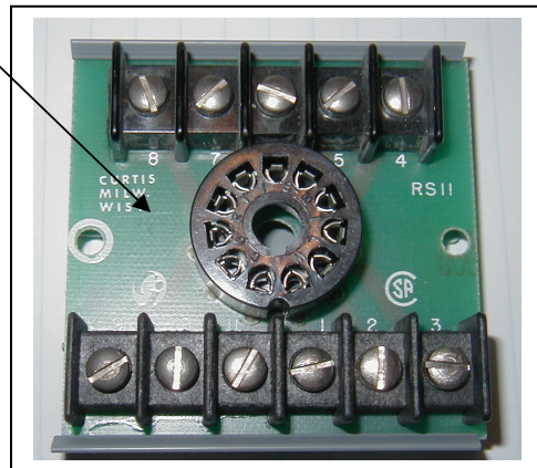
New 11 pin Socket Base MEL-091
